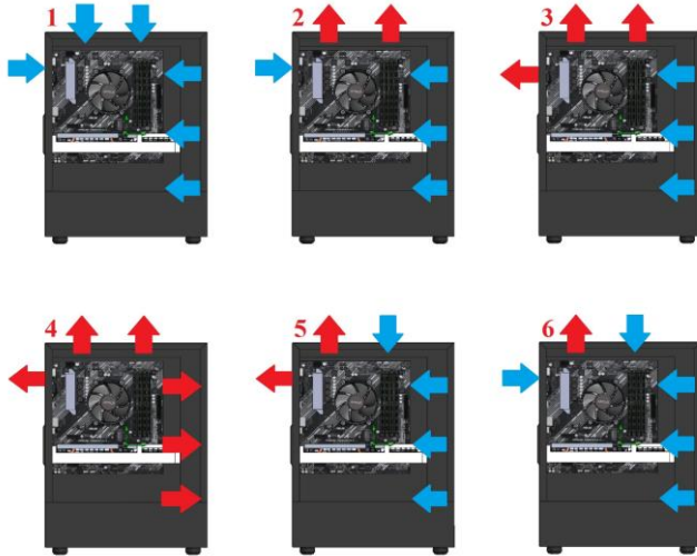
Fig. 3 Configurations used in the simulations with six fans in the XPG VALOR AIR case
