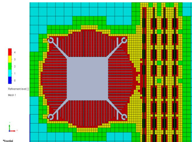
Fig. 5 Fluid mesh in the upper region of the case
