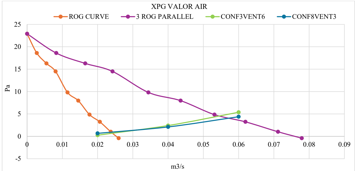
Fig. 7 Intersection of impedance curve and cabinet characteristic curve
