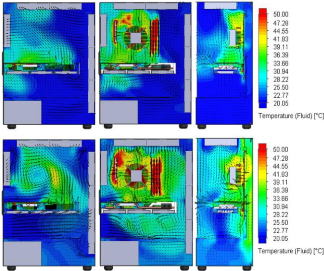
Fig. 8 Air temperature contours with six case fans
