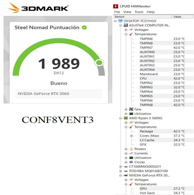
Fig. 13 Results obtained in the performance test with the CONF8VENT3 configuration
