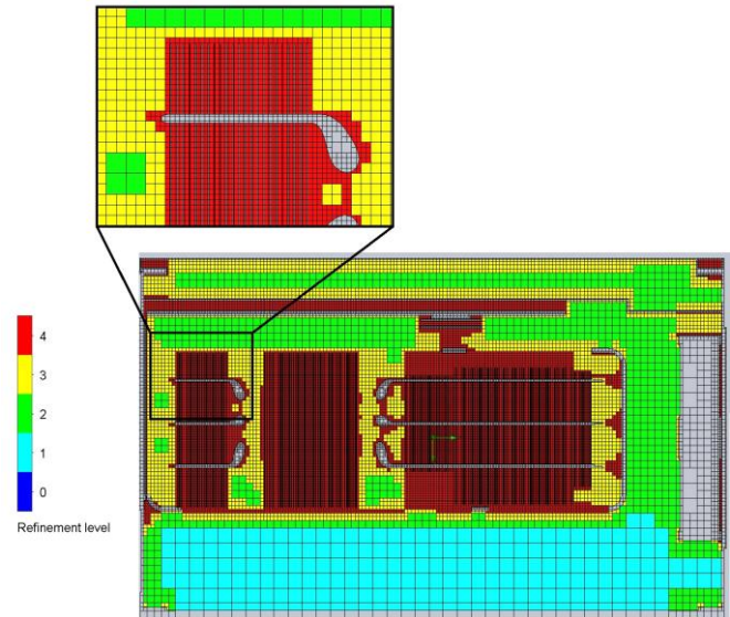
Fig. 6 Fluid mesh in the middle plane of the case graphics card
