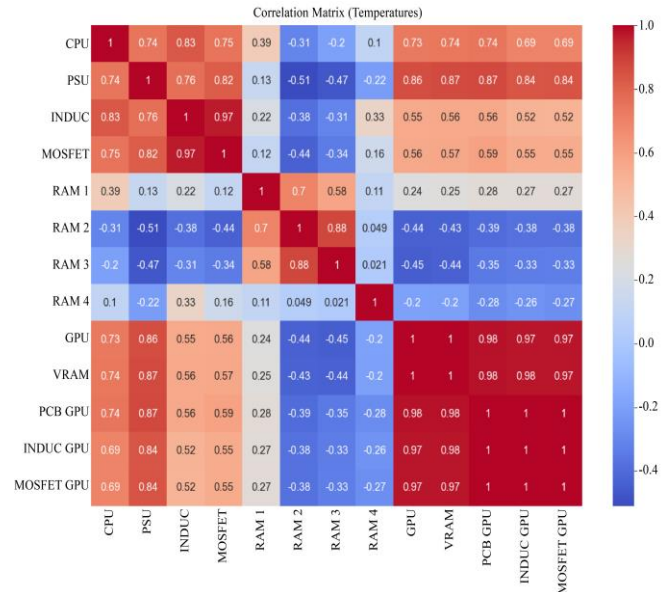
Fig. 10 Correlation matrix of the temperatures of all computer components
