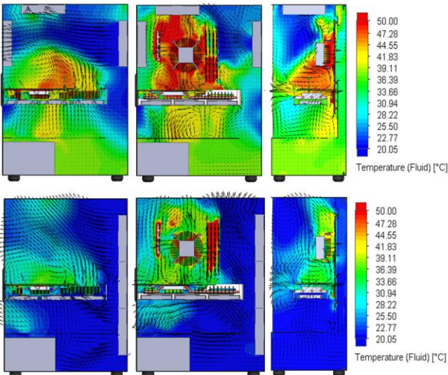
Fig. 9 Air temperature contours with three case fans
