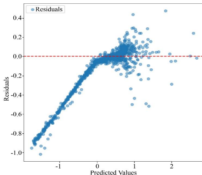
Fig. 10 Residual plot of the CNN model with average pooling algorithm
