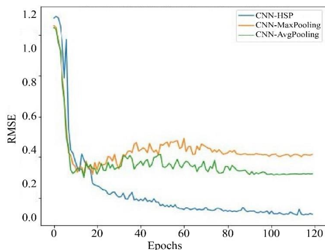
Fig. 4 Root Mean Square Error (RMSE) convergence
