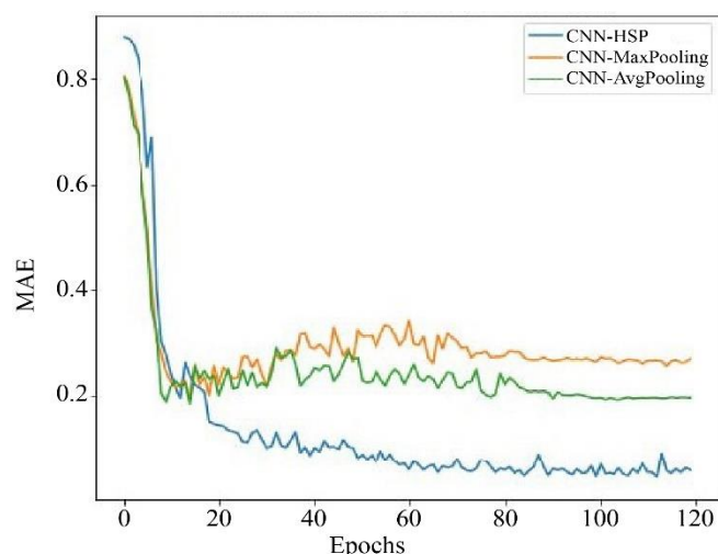
Fig. 3 Mean Absolute Error (MAE) convergence
