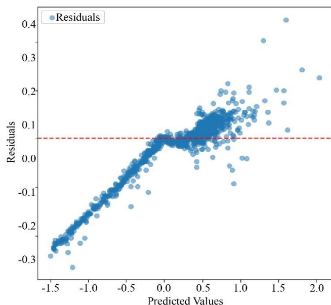
Fig. 9 Residual plot of the CNN model with max pooling algorithm
