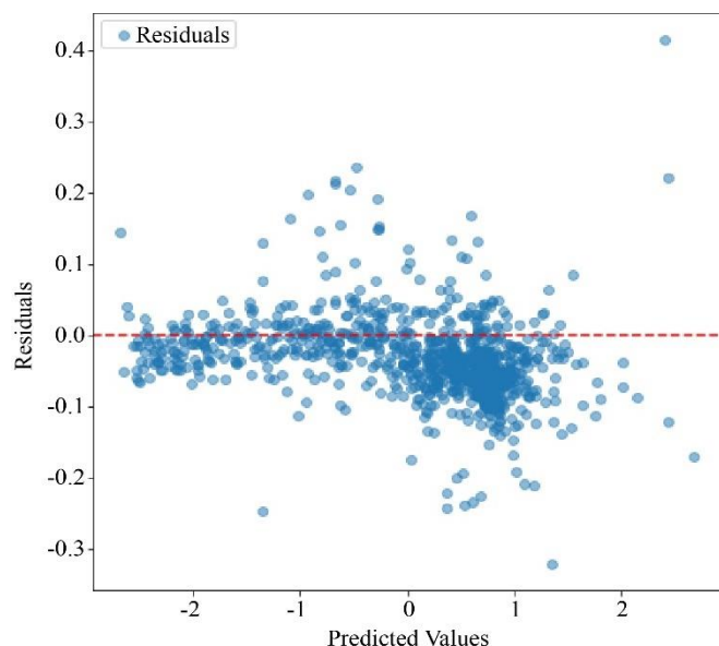
Fig. 8 Residual plot of the CNN model with horizontal sequence pooling algorithm
