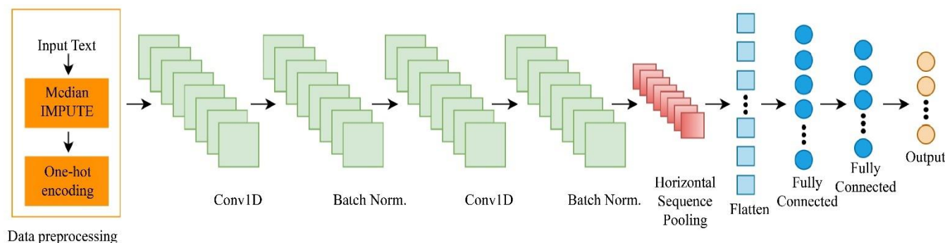
Fig. 1 CNN model with horizontal sequence pooling
