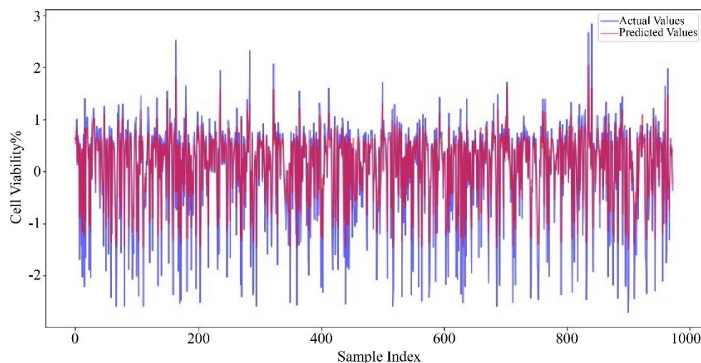
Fig. 6 Actual vs Predicted values of the CNN model with the max pooling algorithm
