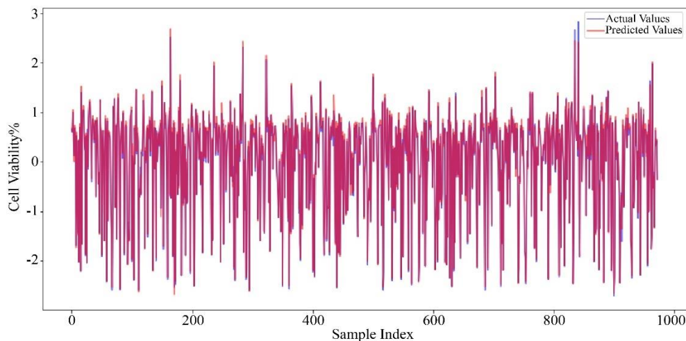
Fig. 5 Actual vs Predicted values of the CNN model with horizontal sequence pooling algorithm
