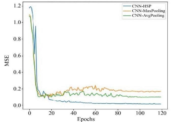
Fig. 2 Mean Square Error (MSE) convergence
