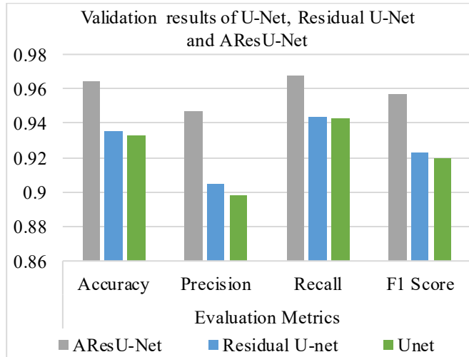
Fig. 9 Validation results of U-Net, residual U-Net and AResU-net
