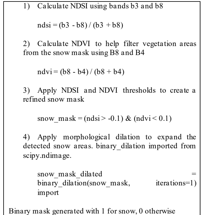
Fig. 4 Steps for snow cover detection using NDVI, NDSI and binary dilation
