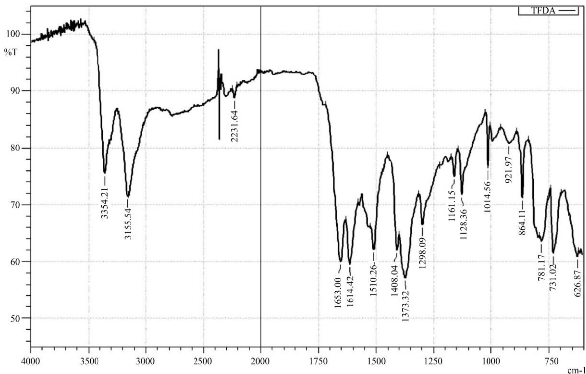
Fig. 7 IR spectrum of the resulting terephthalamide
