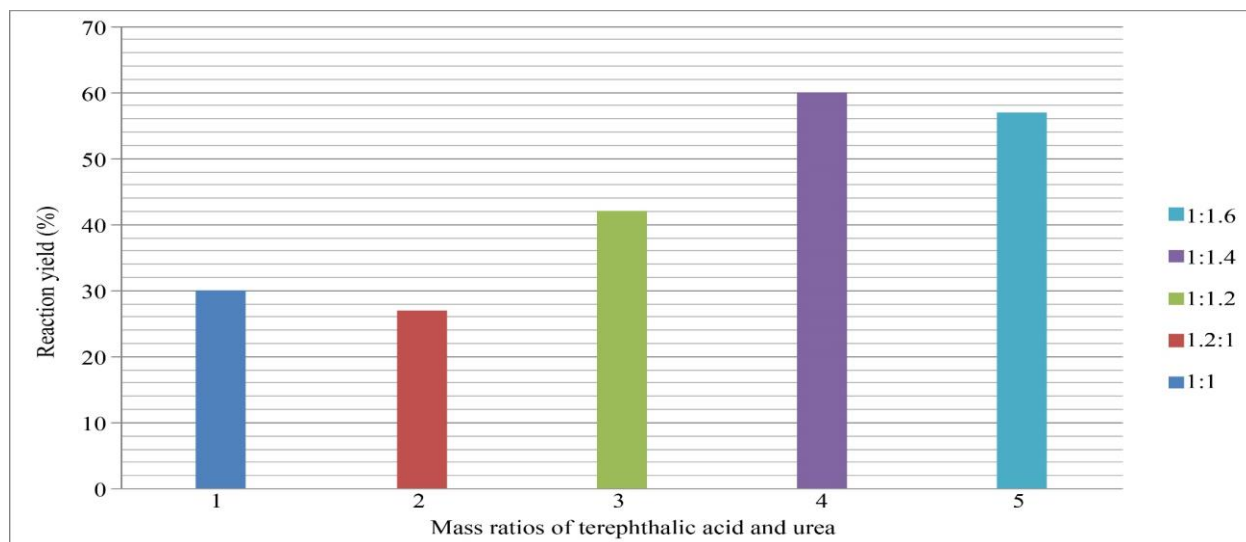
Fig. 1 Relationship between the reaction yield of different mass ratios of terephthalic acid and urea
