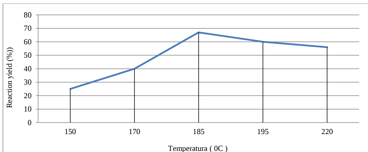
Fig. 2 Temperature dependence of reaction yield
