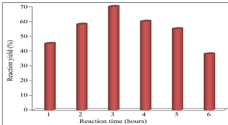
Fig. 4 Time dependence of reaction yield
