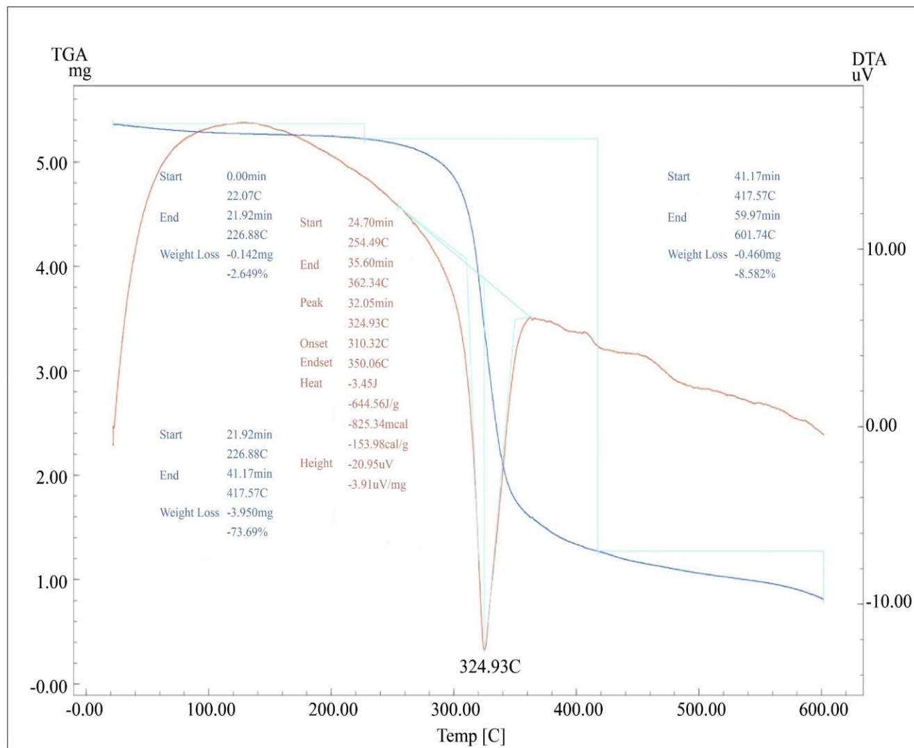
Fig. 9 Derivatogram and thermogravimetric analysis of the resulting terephthalamide sample
