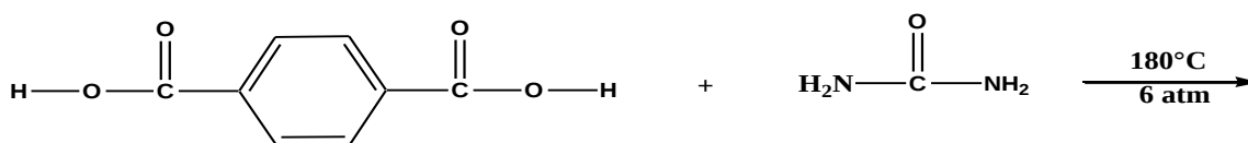
Fig. 5 Effect of catalyst on reaction yield 1. CuCl 2 2. NaCl 3. Ca(OH) 2 4. MgSO 4
