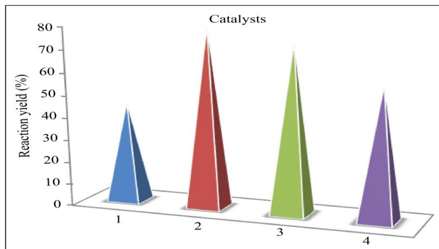
Fig. 5 Effect of catalyst on reaction yield 1. CuCl 2 2. NaCl 3. Ca(OH) 2 4. MgSO 4
