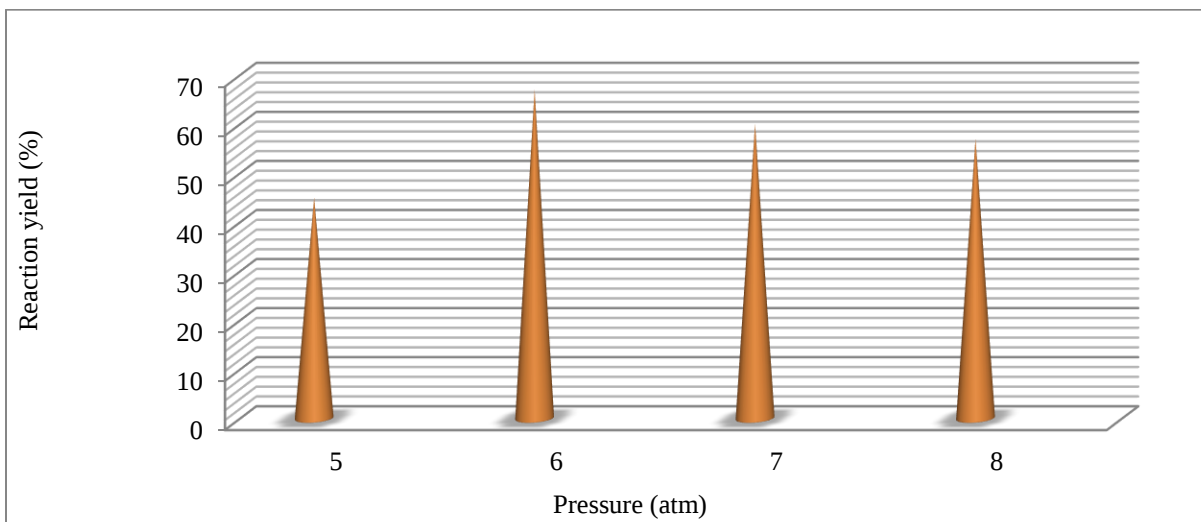
Fig. 3 Pressure dependence of reaction yield
