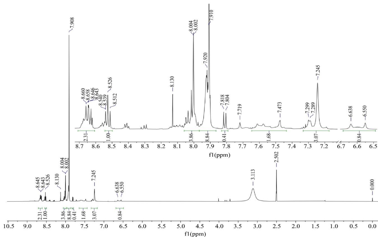
Fig. 10 The result of NMR analysis of the obtained terephthalamide
