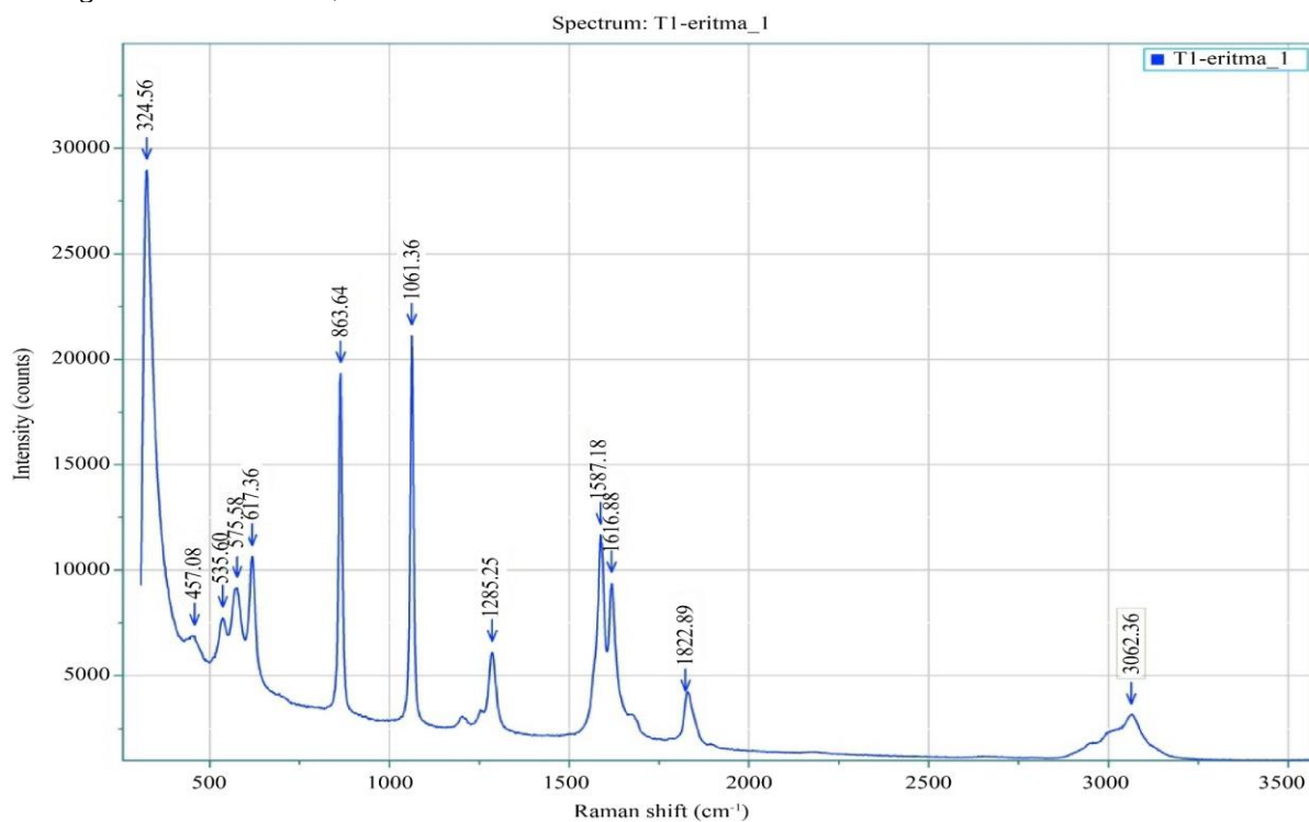
Fig. 8 Raman spectrum of the resulting terephthalamide
