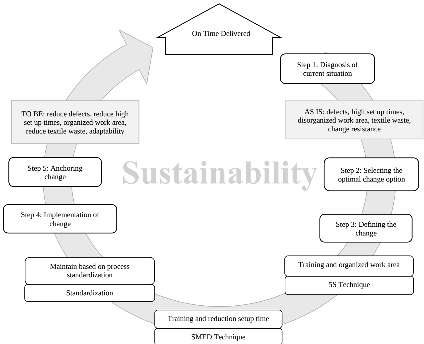
Fig. 1 Proposed method
