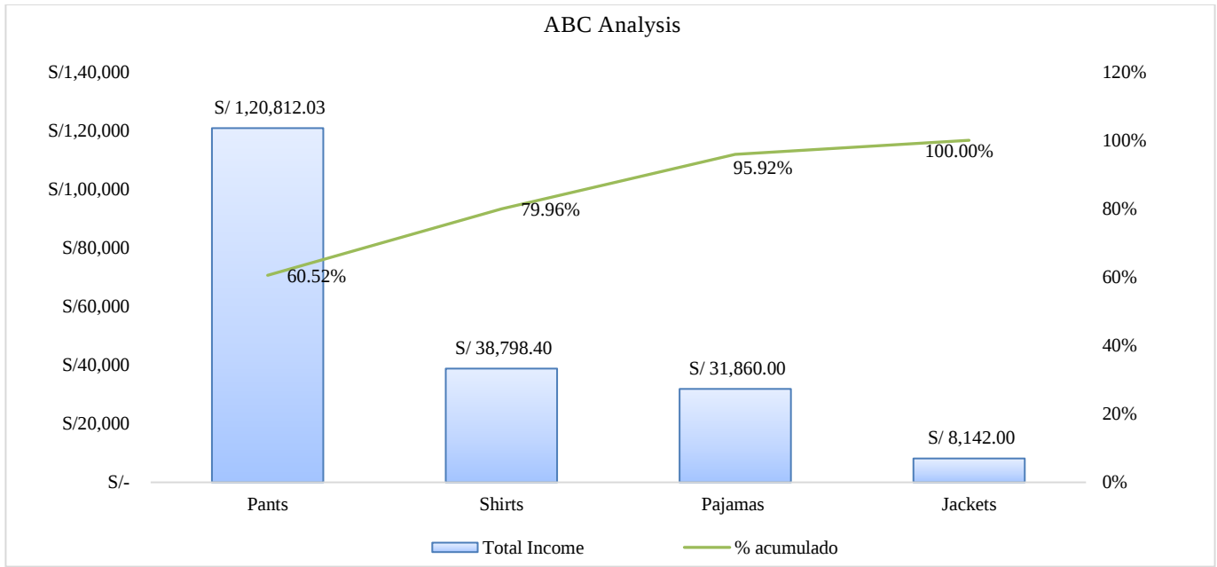
Fig. 3 ABC Analysis
