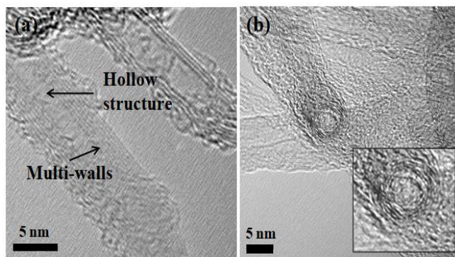
Fig. 5 TEM image of the synthesized carbon nanotubes
